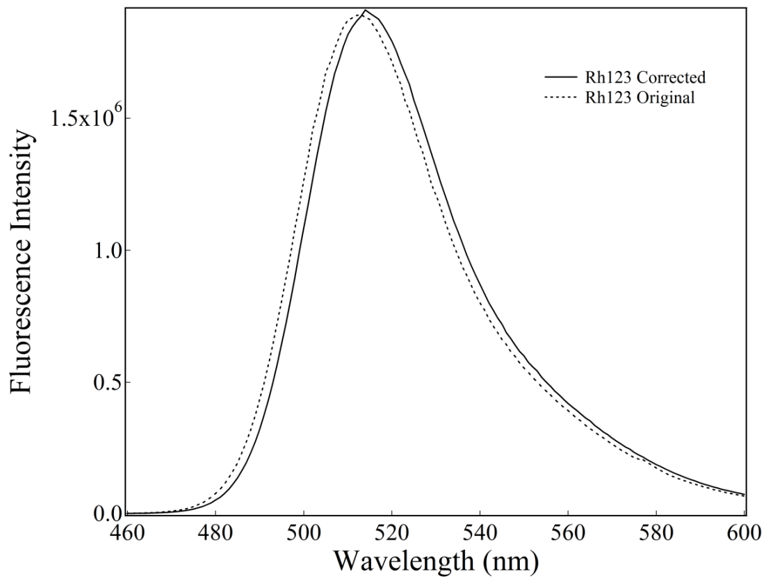
Fig 5.2.1 Uncorrected (dotted line; \lambda_{\text{max}}=512\text{nm} ) and correct (solid line; \lambda_{\text{max}}=514\text{nm} ) fluorescence spectra of Rhodamine 123 in
