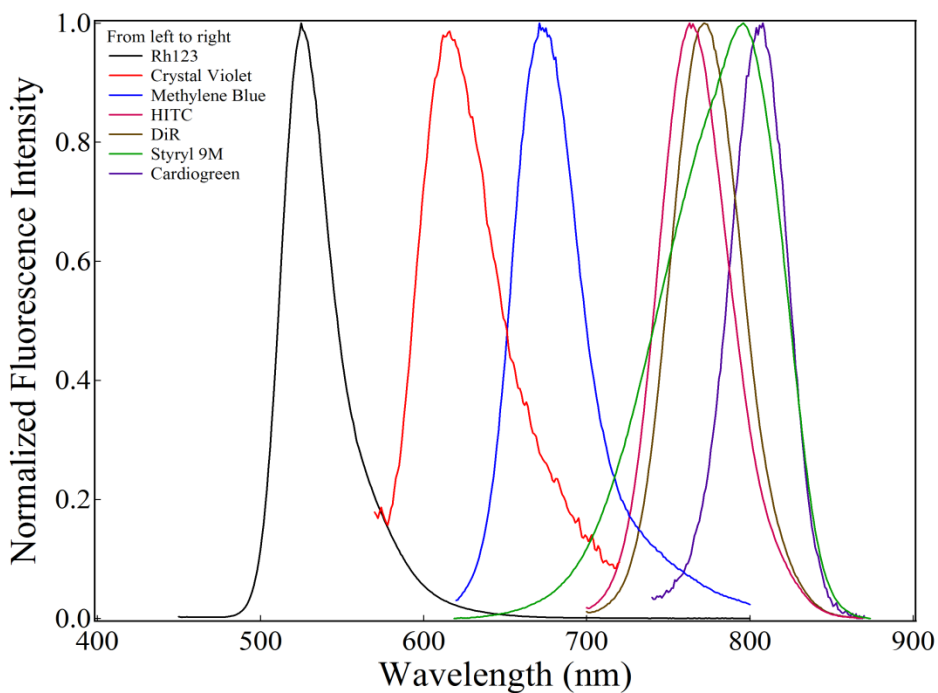
Fig 5.1 Top panel: Absorption spectra of visible and Near-IR absorbing dyes in methanol. From left to right ( \lambda_{\text{max}} , nm): Rh123 (507), Styryl 9M (573), CV (587), MB (654), HITC (740), DiR(748) and Cardiogreen (778). Bottom panel: respective fluorescence spectra in methanol, from left to right ( \lambda_{\text{max}} and \lambda_{\text{excitation}} , nm): Rh123 (525, 440); CV (615, 550); MB (673, 610); HITC (764, 690); DiR (772, 690); Styryl 9M (796, 570); Cardiogreen (808, 690).
