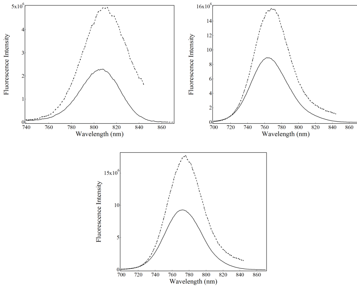
Fig. 5.2.6 Clockwise from the top left panel: Uncorrected (solid lines) and “correct” (dotted lines) spectra of Cardiogreen, HITC
