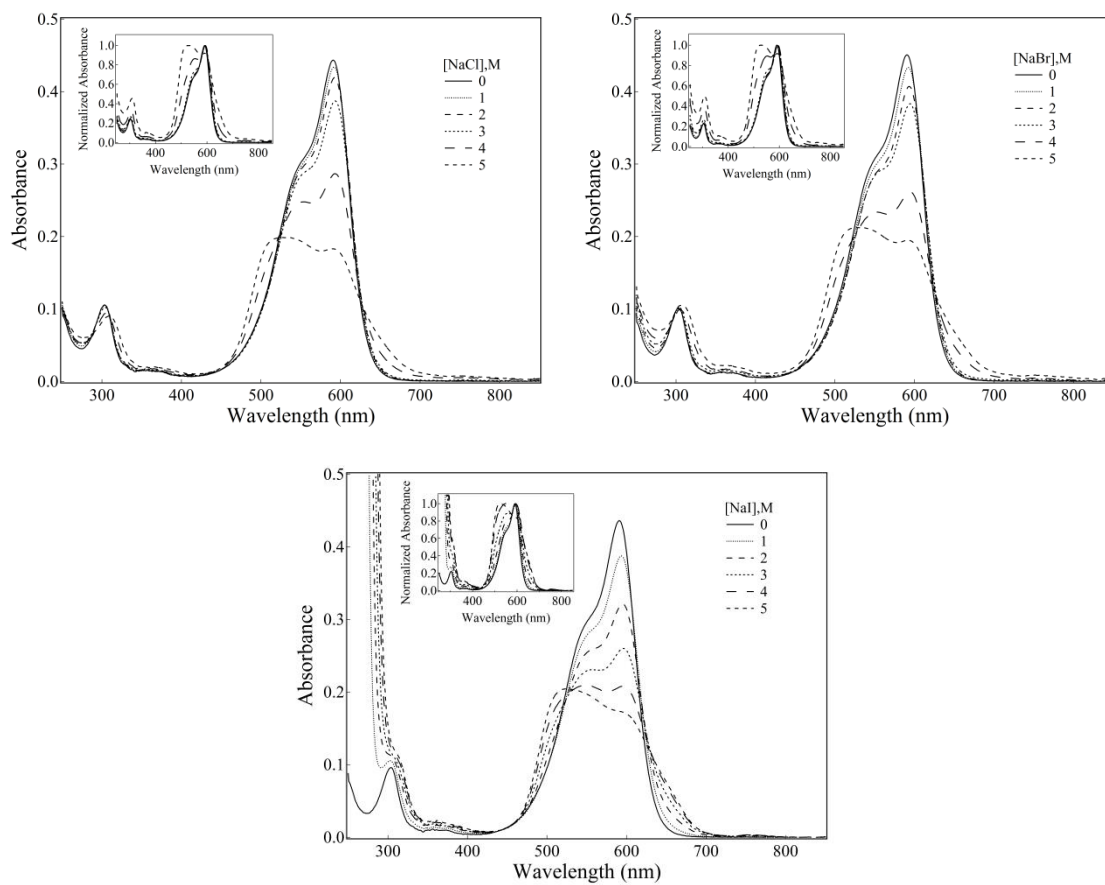
Fig 3.1.2 Salt effects on the absorption spectra of Crystal Violet in aqueous solution. Clockwise, from top left panel: sodium chloride, sodium bromide and sodium iodide. Insets: respective normalized spectra. [CV] = 5 \mu\text{M}
